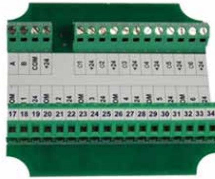
BLUE GIANT REMOTE I/O BOARD PARA GANCHO RETENEDOR TL85-HVR303 YSVR303.
